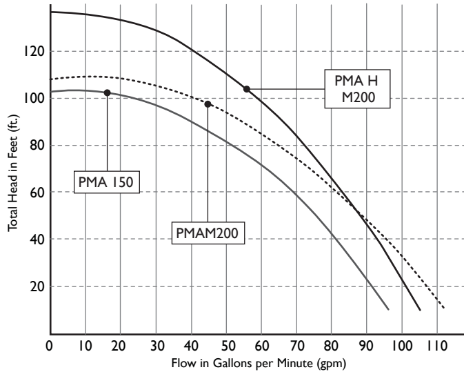
2 hp vs. 1½ hp Pump Performance
